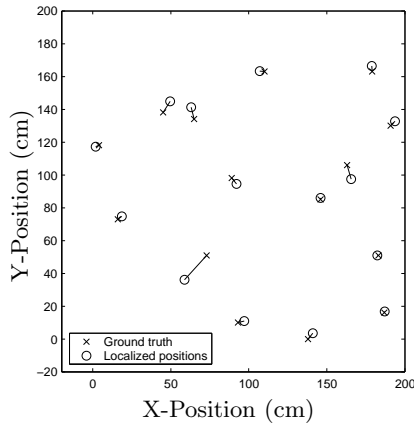
Figure 8: A comparison of node positions as localized by our algorithm to the true positions of the nodes on a physical Cricket cluster. Positions are computed by Phase I of the algorithm, cluster localization. The experiment involved 16 nodes, one of which could not localize; thus only 15 are shown.
